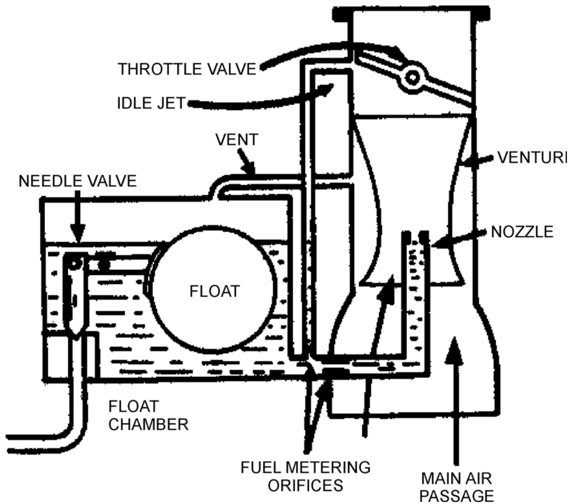
Figure 12C-2 Carburetor Components
