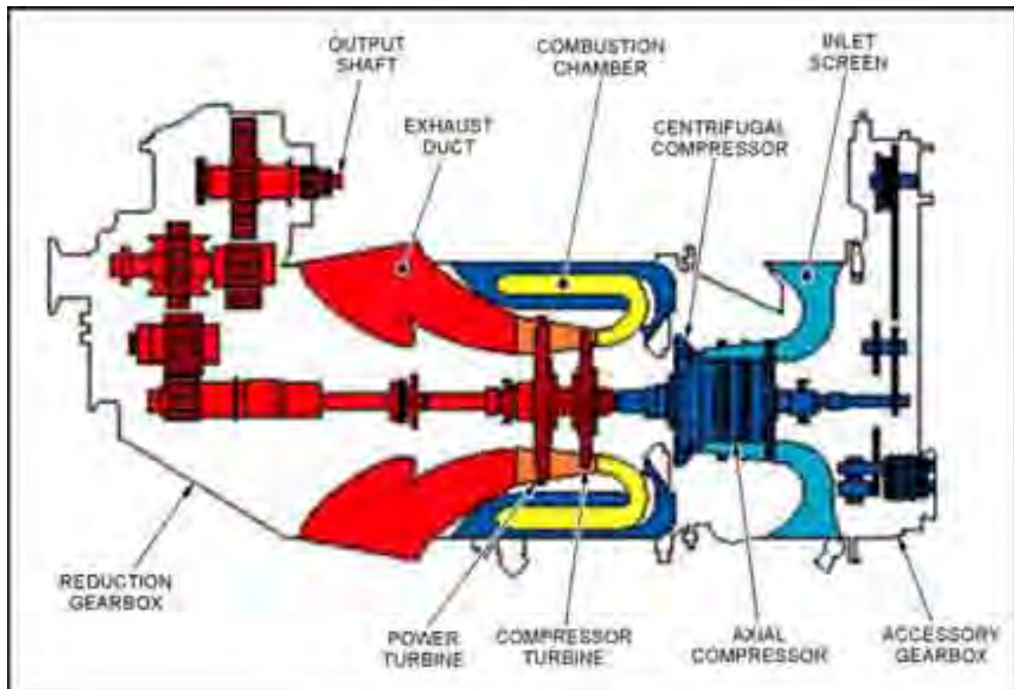
Figure 12V-1 Turboshaft Engine Schematic – Separate Turbines
