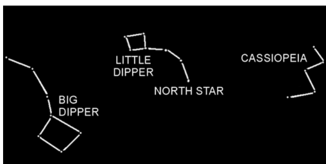
Figure 13-9-3 Little Dipper
